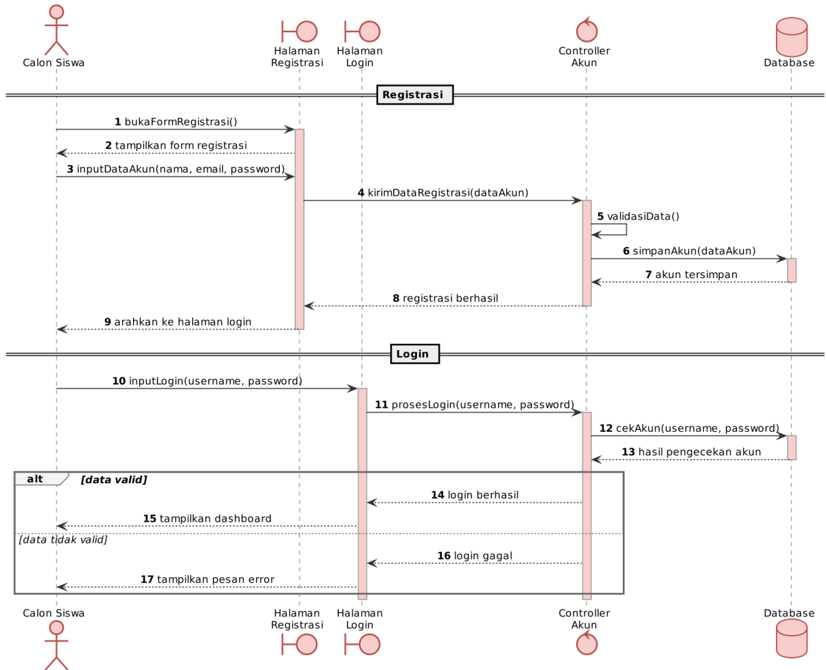
SEQUENCE DIAGRAM REGISTRASI & LOGIN
